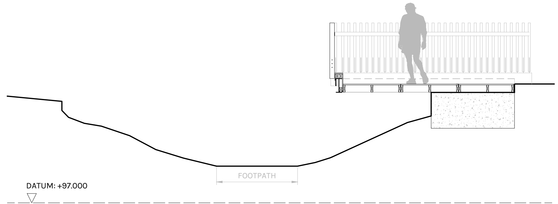
SECTION A-A AT 1:50
